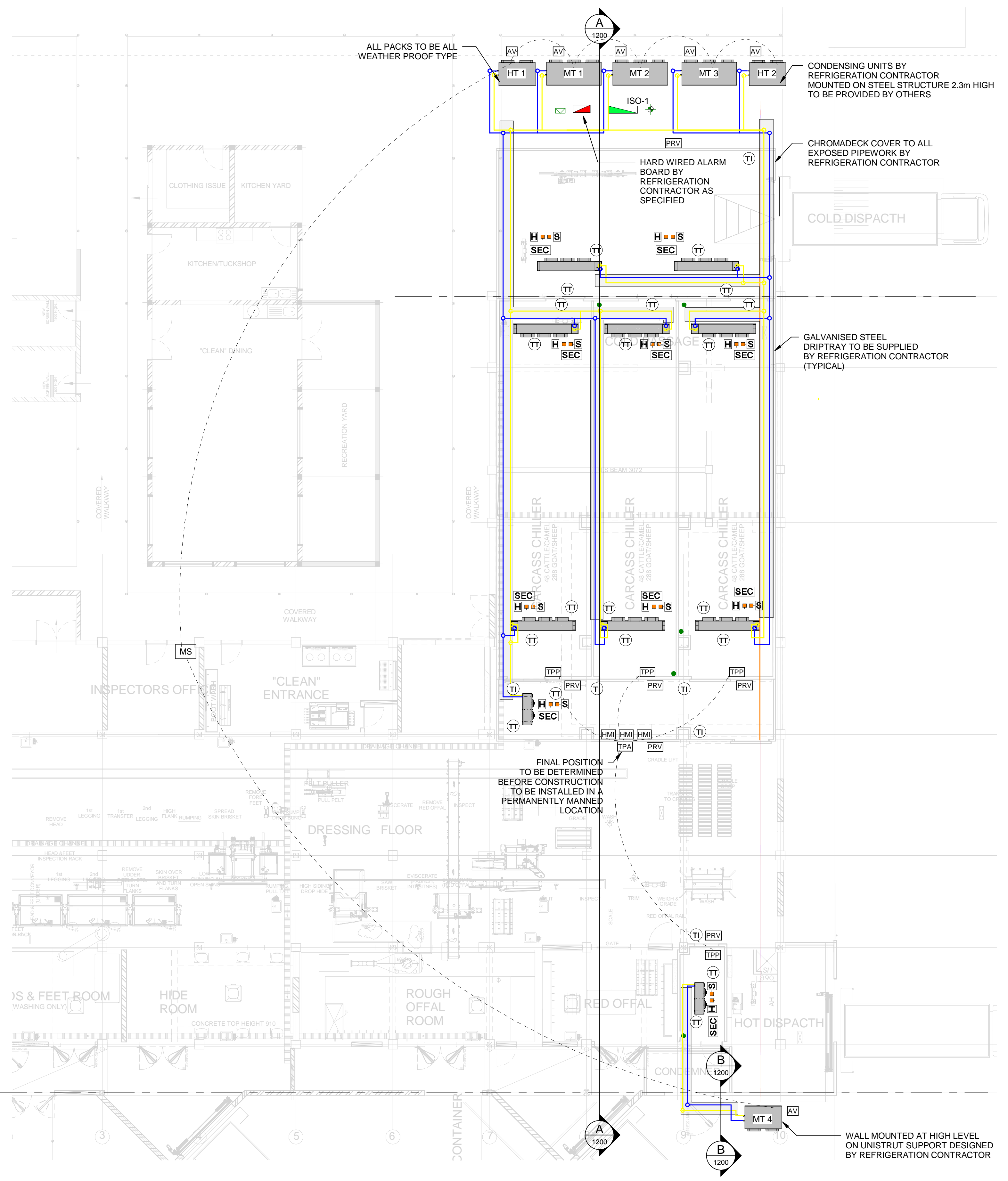
1 PIPE ROUTE LAYOUT 1:100
