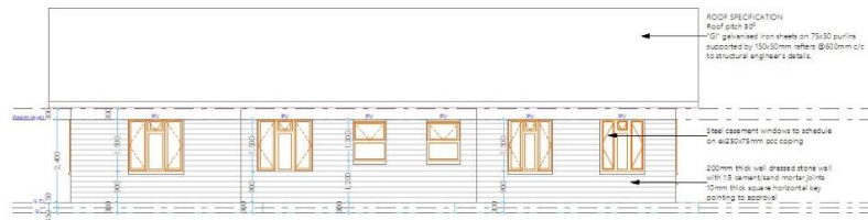
10 Back Elevation 1:100
