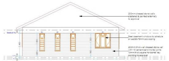
9 East Elevation 1:100
