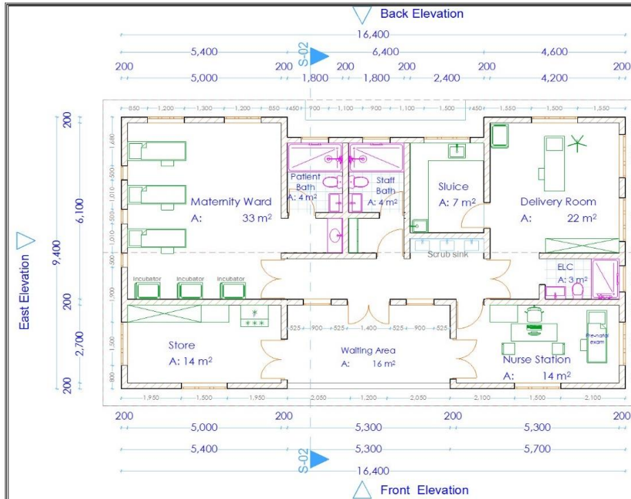
0. Ground Floor (3) 1:75
